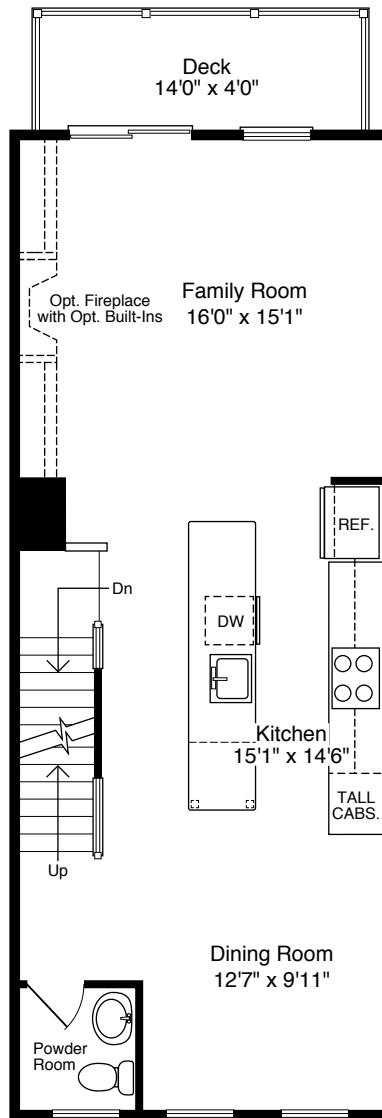
The Fleetwood Alternate Second Floor Plan Window Patterns Vary By Elevation
