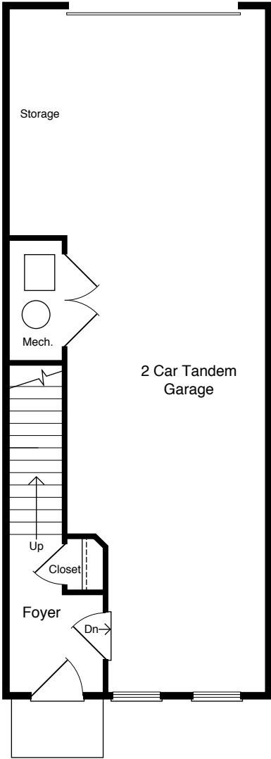
The Fleetwood Ground Floor Plan Window Patterns Vary By Elevation
