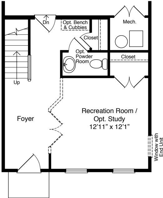
The Rockland Ground Floor Plan w/Opt. Powder Room Window Patterns Vary By Elevation
