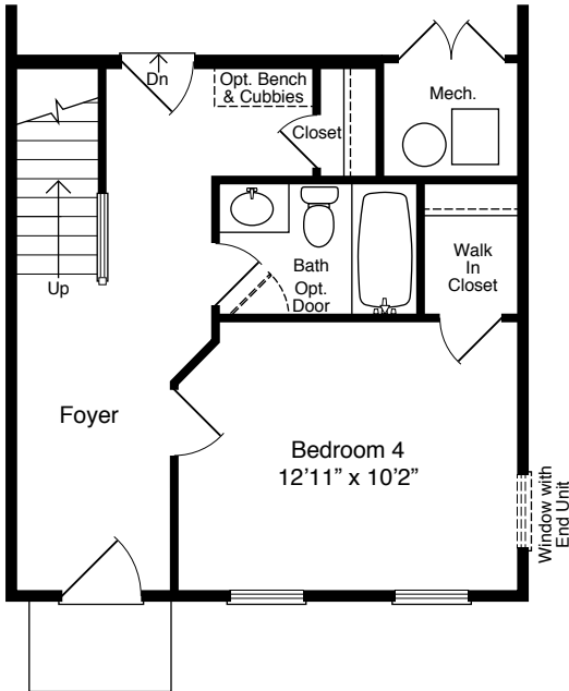
The Rockland Ground Floor Plan w/Bedroom 4 and Full Bath Window Patterns Vary By Elevation
